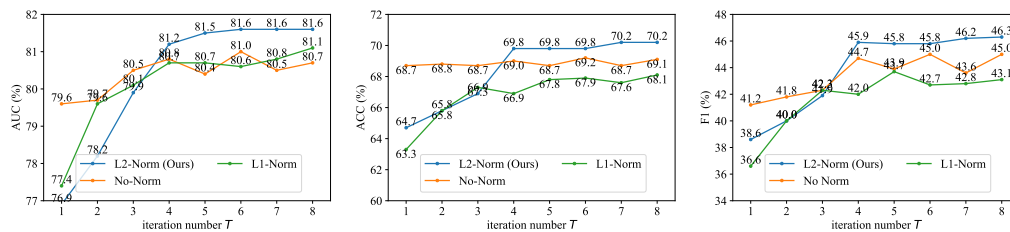
Figure 6: Impact of severity base normalization on generalized medical grading performance. Evaluation metrics AUC, ACC and F1 are presented in percentage (%). Domain-1 and Domain-2 in the Fatigue Fracture Grading Benchmark are used as the source and unseen target domain, respectively. Better zoom in to view.
