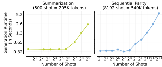
Figure 12: Per-Output runtime as we increase shots , averaged across the test set and multiple seeds, on (left) summarization and (right) parity prediction. When computing the next token, we still have to attend to the fixed many-shot prompt, even if KV is cached.
