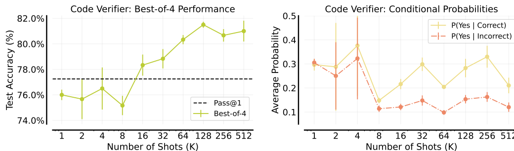
Figure A.4: Learning Verifiers In-Context for checking correctness of GSM8K code solutions. Error bars denotes standard error of mean over 3 seeds. See Figure A.11 for a 2-shot prompt. Best-of-N accuracy. (Left) Average accuracy of top-ranked code solutions (among 4 solutions) based on the verifier score on 200 GSM8K test problems. Best-of-4 selection with 128-shot bridges the gap between Pass@1 accuracy of 77.25% and Pass@4 accuracy of 90% with Gemini 1.0 Pro model. Verifier Confidence. (Right) Conditional Probabilities of the Yes token P(Yes) from the verifier, averaged over all correct and incorrect solutions on test problems.
