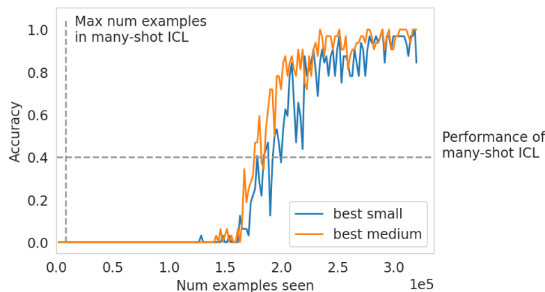
Figure A.19: For the sequential parity task, training a transformer from scratch does not meet 8192-shot ICL performance (dashed lines) until 20\times the number of examples. We trained two transformers on the sequential parity task (from §4.2). The smaller model was the size of GPT-2 Small, with 12 layers and 768 embedding dimension. The larger model was the size of GPT-2 Medium, with 24 layers and 1024 embedding dimension. We trained using a linear warmup and square root decay schedule, sweeping max learning rate values [1e-5, 5e-5, 1e-4, 5e-4, 1-e3] and num warmup steps [50, 100, 500, 1000, 5000]. The best values for both models (fastest learning) were max_lr=1e-4, warmup_steps=1000.
