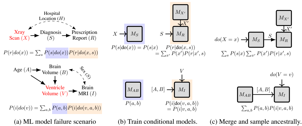
Figure 1: (Top: x-ray to report generation task) (a) \text{do}(X = x) removes the X \leftrightarrow R bias and makes the generation of R domain invariant. P(r|\text{do}(x)) is factorized into c-factors and (b) conditional models ( \{M_{V_k}\}_k ) are trained for each factor (shown as boxes). (c) The intervened value X = x is propagated through the merged network and samples from the P(r|\text{do}(x)) are generated.
