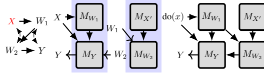
Figure 2: \leftrightarrow :Unobserved. Left blue samples from P_{x, w_2}(w_1, y) = P(w_1|x) P(y|x, w_1, w_2) . Right blue samples from P_{x, w_1}(w_2) = \sum_{x'} P(x') P(w_2|x', w_1) . Joint network samples from P_x(y) .
