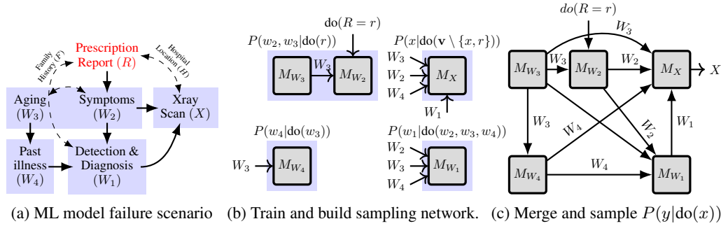
Figure 7: do(R = r) removes the R \leftrightarrow X bias and makes prediction of X domain invariant. ID-GEN factorizes P(\mathbf{v}|do(r)) into four factors and trains conditional models ( \{M_{V_i}\}_i ) for each (blue shades). The intervened value R = r is propagated through the merged network to generate all other variables.
