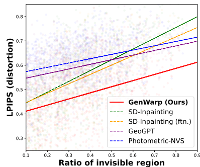
Figure 13: Comparison of LPIPS with other methods regarding ratio of invisible region. We measure LPIPS between generated views and GT target views, following GeoGPT [36]’s evaluation protocol.
