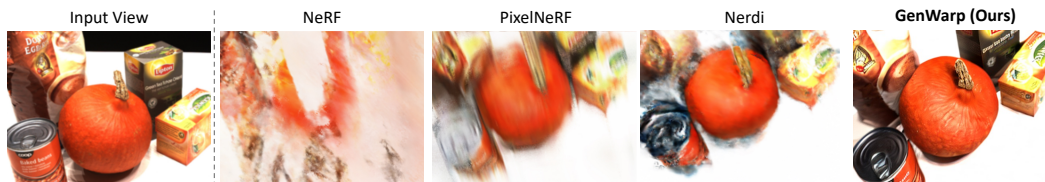
Figure 15: Comparison with reconstruction-based methods on DTU dataset [18]. Note that our model used here is not trained on DTU dataset.
