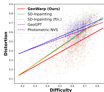
Figure 8: Comparison on various viewpoint changes.
