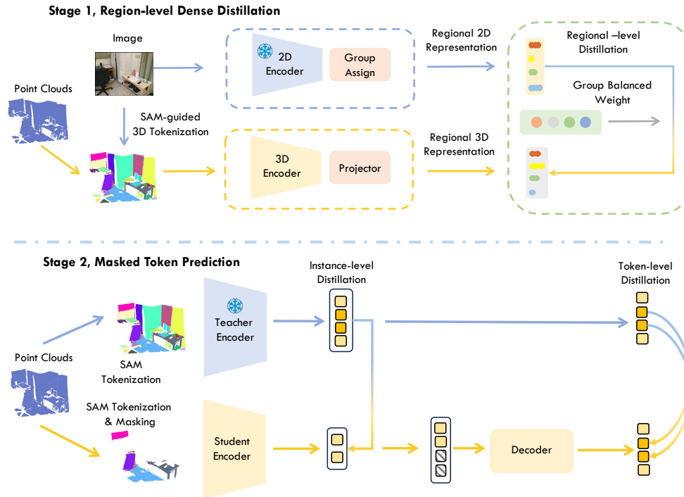
Figure 2: Overall framework of the proposed method. Our method introduces a two-stage masked token prediction framework for learning from foundation models. In the first stage, we input complete point clouds and leverage SAM masks to guide the point cloud tokenization, thereby seamlessly aligning the 2D and 3D region-level features for dense prediction. A group-balanced weight is applied during distillation to prevent bias towards the head representations. In the second stage, we freeze the models trained in the first stage and have the student models predict instance-level features and masked tokens obtained from the teacher models.
