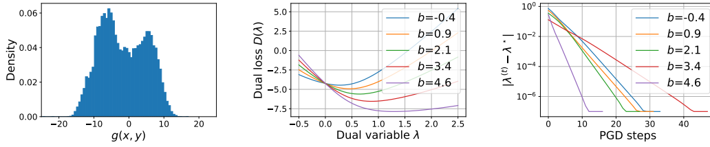
Figure 1: An illustration of the dual properties with 128 responses drawn from the Alpaca-7b-reproduced model operating over 1000 prompts from the PKU-SafeRLHF-30K dataset. (Left) The empirical distribution of the safety scores. (Middle) The dual landscape with respect to varying margin b . (Right) The convergence of PGD with a constant step size of one and initialization \lambda^{(0)} = 1 .
