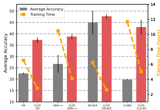
Figure 4: Comparison of different methods for S-CIFAR-10 dataset using Nvidia Jetson Orin NX with a buffer size of 125. When combined with various CL methods, CLFD significantly reduces training time while simultaneously enhancing model accuracy.
