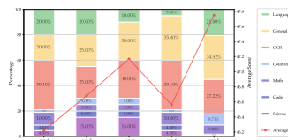
Figure 9: Exploring instruction tuning data mixture ratios.
