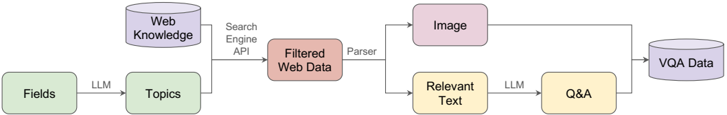
Figure 15: Targeted Internet Data Collection Engine. We build a targeted internet data engine to collect high-quality and large-scale multimodal instruction tuning data for domains like knowledge.
