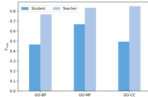
Figure 4: Performance comparisons of the teacher and student of ProtGO on GO term prediction.
