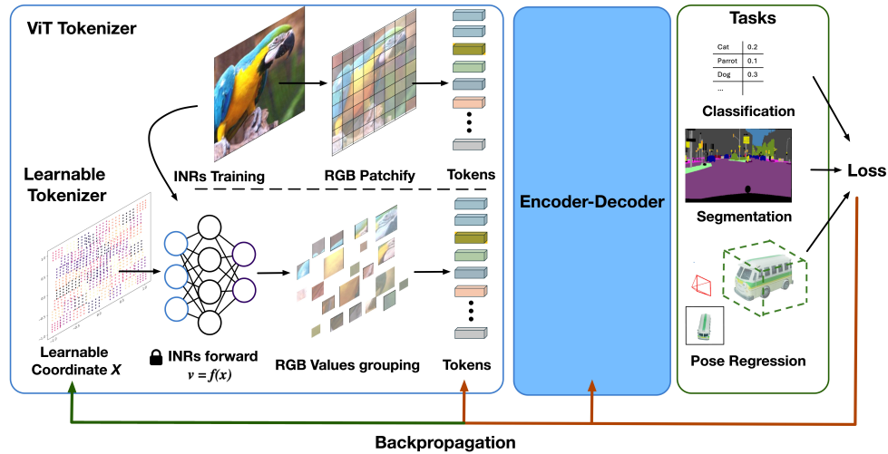
Figure 3: Illustration of learnable tokenizer. Instead of retrieve RGB value from images we query learnable coordinates to pre-trained frozen INRs and grouping RGB values to create tokens. Note that during backpropagation the Coordinate x will also be jointly optimized with ViT modules .
