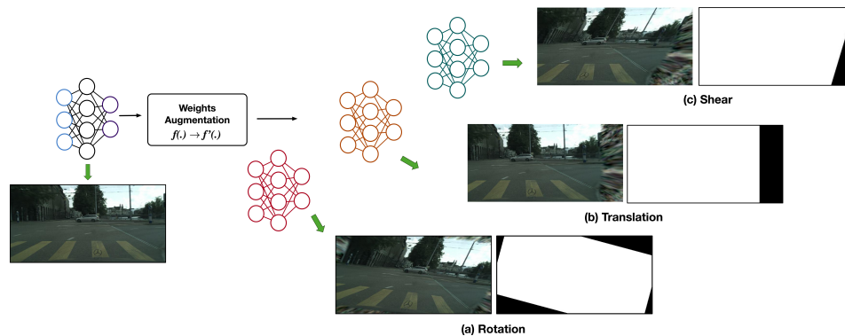
Figure 14: Masking out-of-range values: We implement zero-padding by applying same geometric transformation for a binary mask and we show examples for (a)rotation, (b)translation and (c)shear operation. Out-of-range RGB values are clearly visible in the bottom right corner of the transformed image.
