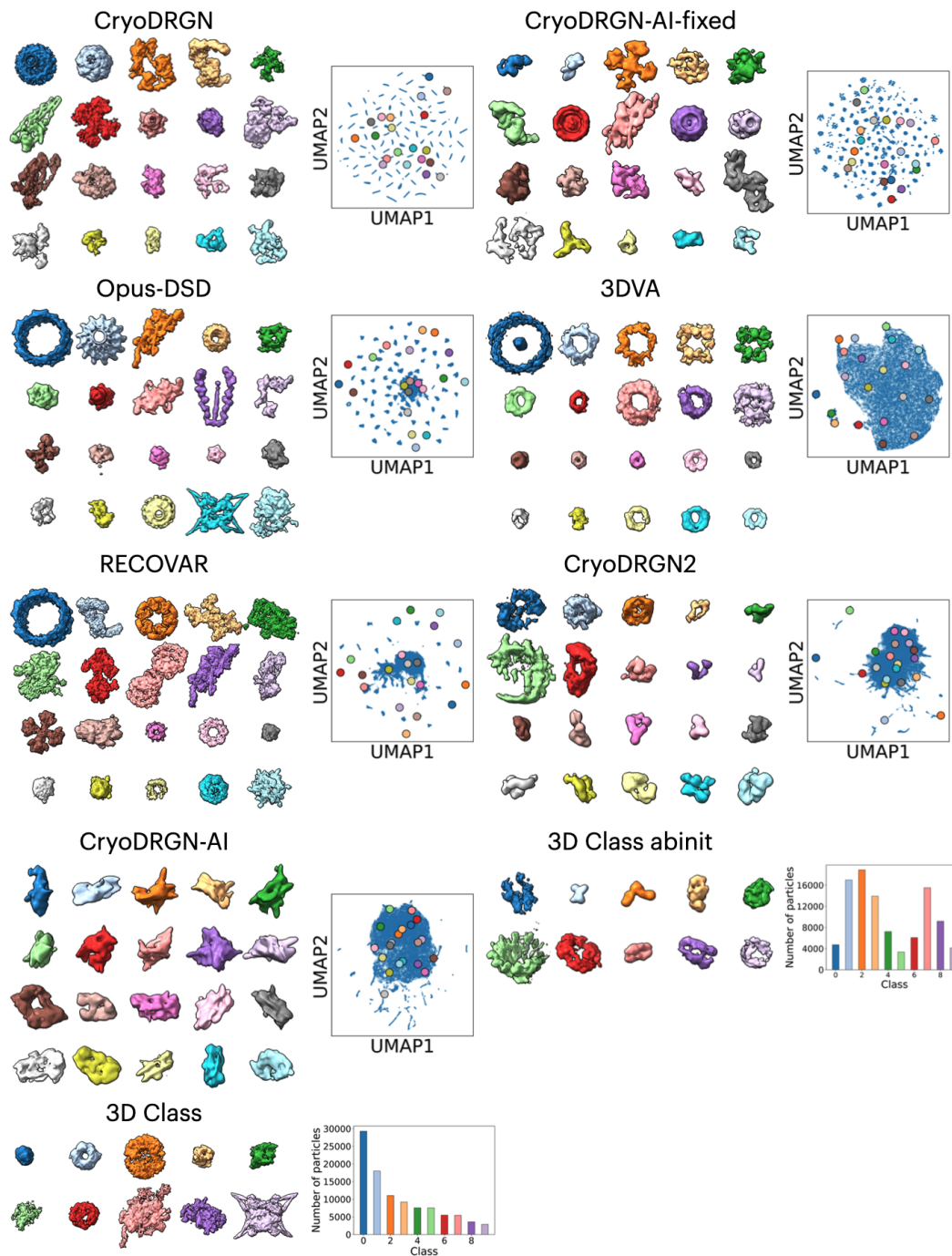
Figure S21: Qualitative Results (Tomotwin-100). Representative volumes and UMAP visualization of the latent embeddings for each method. Volumes correspond to k -means cluster centers with k=20 and are colored according to the associated point. Class volumes and particle counts are shown for 3D Classification.
