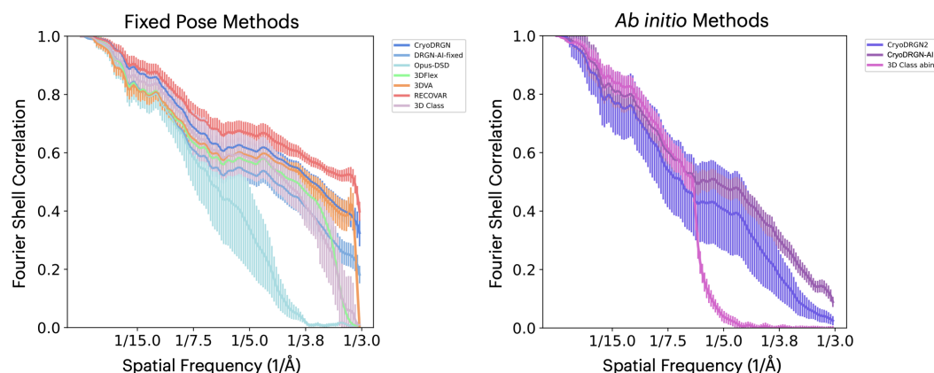
Figure S12: Per-Image FSC for Spike-MD. Each curve shows the average FSC curve across 100 sampled images with error bars indicating the standard deviation.
