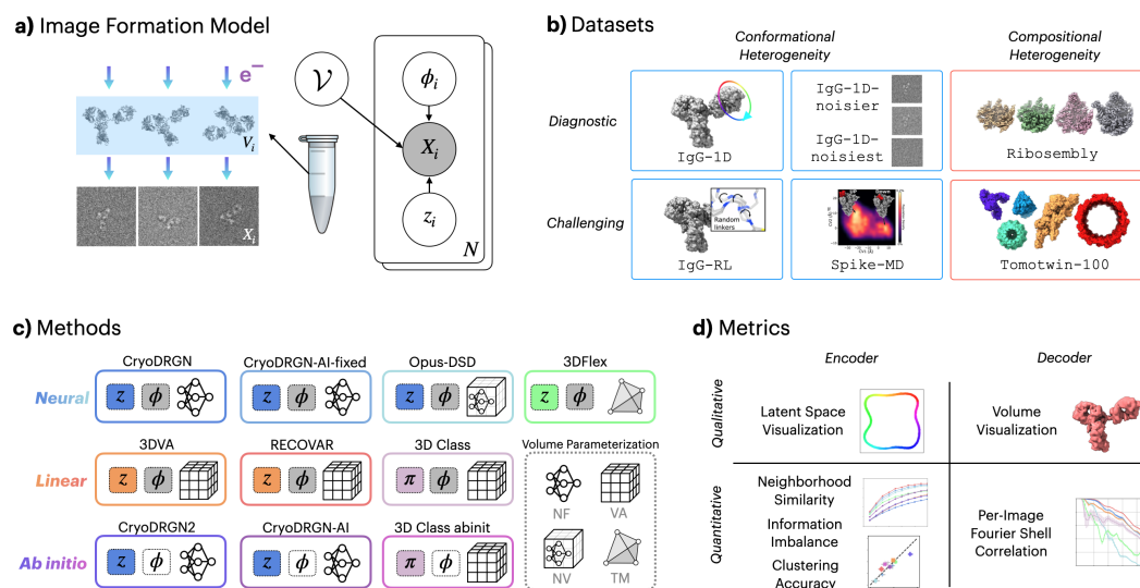
Figure 1: Overview of CryoBench. a) Image formation model. In cryo-EM, each image X_i captures a molecule V_i projected at an unknown pose \phi_i . A latent variable z_i models the conformational space \mathcal{V} that describes the heterogeneity among the set of molecules \{V_i\} . b) Datasets. CryoBench includes 5 synthetic datasets of varying difficulty, characterized by heterogeneity arising from conformational (i.e. shape) or compositional (i.e. identity) changes. c) Methods. Methods can be grouped into using either a continuous latent variable z or discrete latent variable \pi for modeling heterogeneity. Hidden variables assumed to be known are shown in gray. Volumes are represented as a neural field (NF), voxel array (VA), neural volume (NV), or tetrahedral mesh (TM). Generative models are colored blue for nonlinear neural methods; orange for linear generative models, pink for mixture models; and green for density-preserving motion models. d) Metrics. Summary of metrics used to assess both latent inference and volume reconstruction quality.
