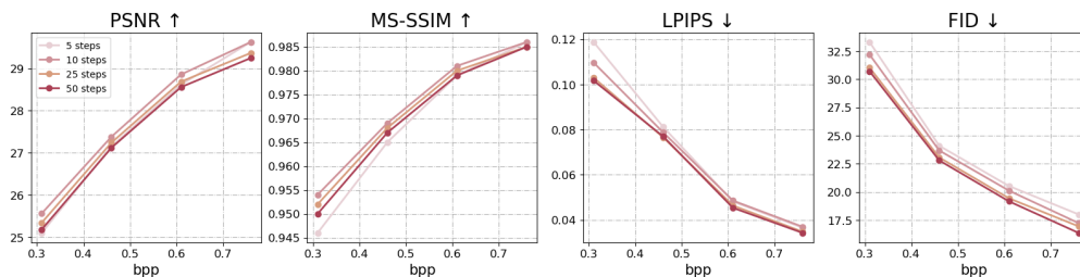
Figure 8: Compression performance with different numbers of decoding step.
