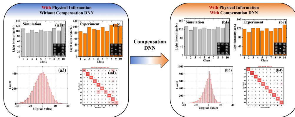
Figure 5: The simulation and experiment result with and without compensation DNN on MNIST dataset, maintaining with quantifiable physical information. (a1,b1) The simulational light intensity in ten classification regions is depicted in the inset. (a2,b2)The experimental light intensity in ten classification regions is depicted in the inset. (a3,b3) Histogram of light intensity difference \Delta I between simulation and experiment. (a4,b4)Experimental confusion matrix.
