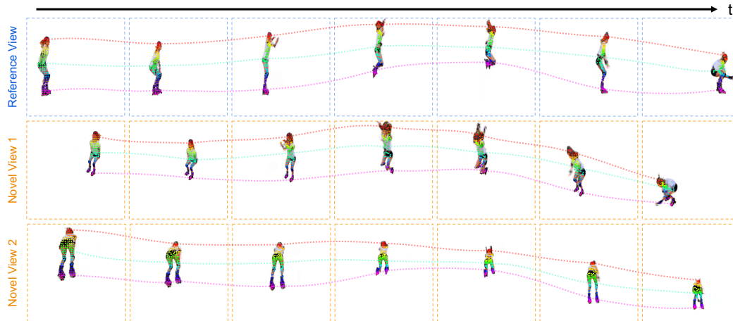
Figure 8: Gaussian Motion Visualizations. We visualize the Gaussian trajectories in the reference view corresponding to the video as well as in multiple novel views. The rendered Gaussians are sampled independently for each view. DreamScene4D can produce accurate motion in different camera poses w/o explicit point trajectory supervision.
