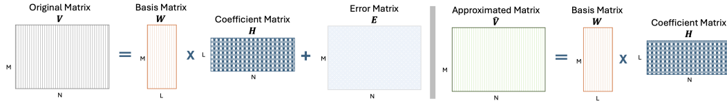
Figure 1: Formulation of Nonnegative Matrix Factorization (NMF)
