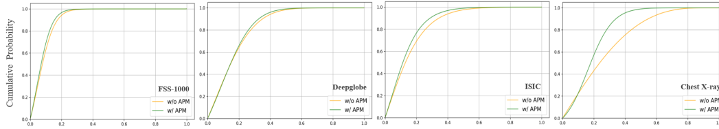
Figure 6: Cumulative distribution function (CDF) of inter-channel correlations. After passing through APM, the CDF curve shifts to the left, indicating a decrease in inter-channel correlations.
