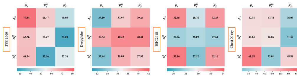
Figure 1: For a model already trained on the source domain, we simply filter out different frequency components and plot mIoU against the maintained ones of images. P denotes Phase, A denotes Amplitude, H denotes High Frequency, and L denotes Low Frequency. We can see the performance is significantly improved in most cases compared with the baseline ( A_x, P_x ), even as high as 14% on the Chest X-ray dataset ( A_x^L, P_x ). In this paper, we delve into this phenomenon for an interpretation, and propose a lightweight frequency masker for efficient cross-domain few-shot segmentation.
