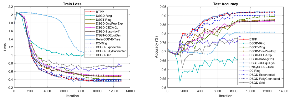
Figure 3: Train loss and test accuracy of different algorithms for training CNN on MNIST, where the dotted lines correspond to the algorithms whose degrees are not \Theta(1) . We perform BTPP with B = 2 , ODEquiDyn with \eta = 0.5 , Base- (k + 1) with k = 2 , and RelaySGD on a binary tree graph for fairness.
