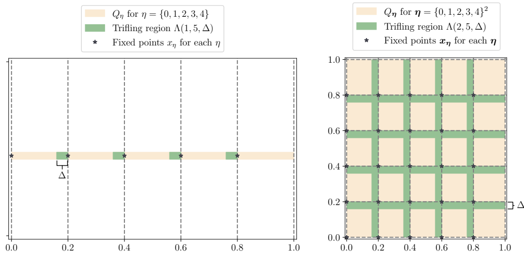
Figure 2: An illustration of localization. The left panel demonstrates the localization \bigcup_{\eta} Q_{\eta} for K = 5 and d = 1 . The right panel shows the case of localization for K = 5 and d = 2 . The “volume” of the trifling region \Lambda(d, K, \Delta) is no more than dK\Delta .
