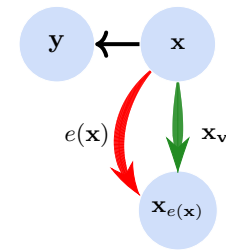
Figure 2: Intuition for encoding: There are two ways the information in the inputs \mathbf{x} about the label \mathbf{y} is transmitted to the explanation \mathbf{x}_{e(\mathbf{x})} : (1) through the values in the explanation and (2) the selection e(\mathbf{x}) (in red). When the latter happens, the explanation is said to be encoding .
