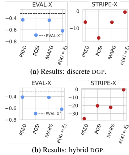
Figure 4: EVAL-X and STRIPE-X scores of the 3 encoding constructions and the non-encoding constant explanation ( e(\mathbf{x}) = \xi_1 ), for both DGPs. EVAL-X, being only a weak detector, assigns suboptimal scores to all encoding explanations ( < ), but scores some encoding explanations above the constant explanation. On the other hand, STRIPE-X, being a strong detector, pushes down the scores of all the encoding explanations below that of the non-encoding constant explanation that always selects \mathbf{x}_1 .
