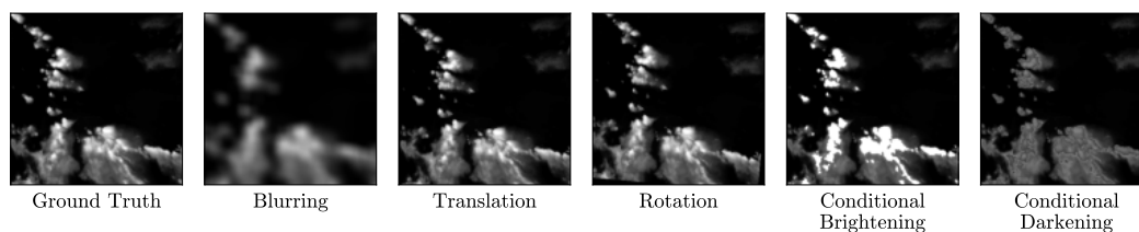
Figure 10: Visualization of different transformation techniques applied on the radar image.
