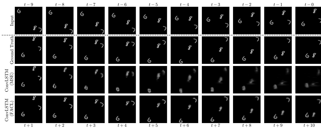
Figure 6: Output frames of ConvLSTM trained with MSE and FACL on N-body-MNIST.
