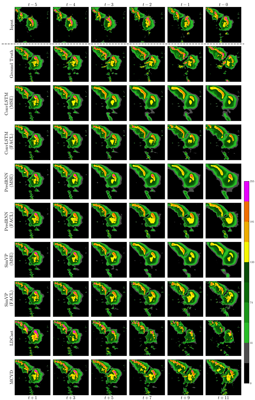
Figure 12: Output frames of the experimented model trained with different losses on SEVIR.
