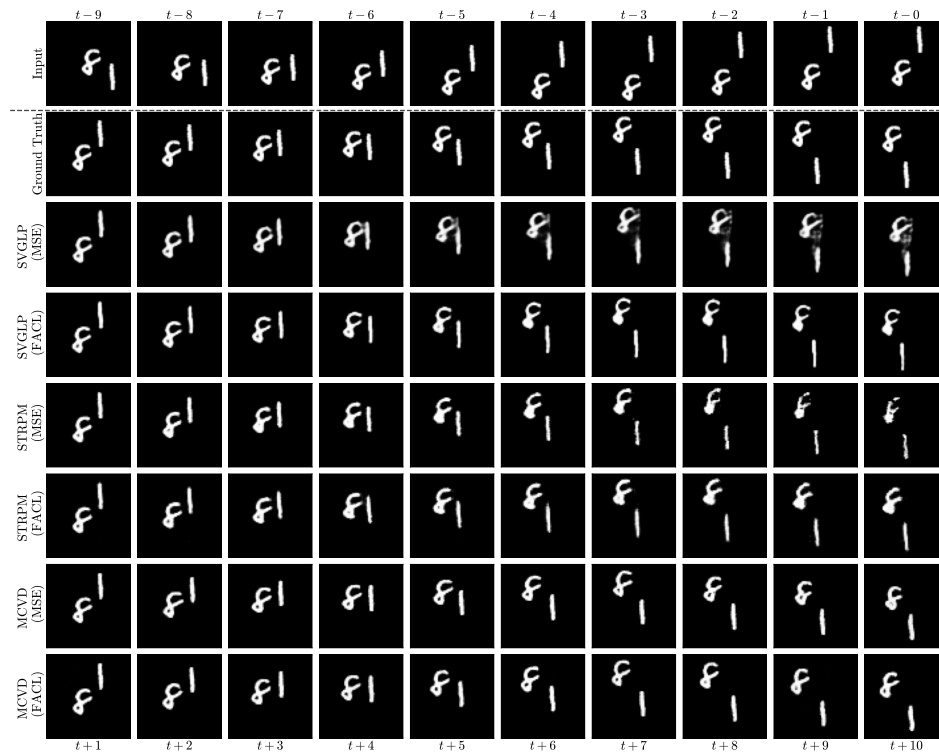
Figure 9: Output frames of video generative models trained with different losses stated in Table 11 on Stochastic Moving-MNIST.
