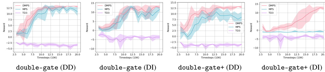
Figure 4: Episodic Returns in double-gate and double-gate+
