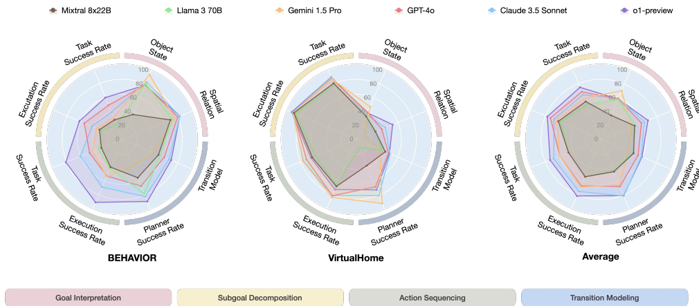
Figure 23: Performance Overview: Tasks in BEHAVIOR require longer sequences of actions and complex subgoal decomposition, while VirtualHome presents greater challenges in understanding environmental states.
