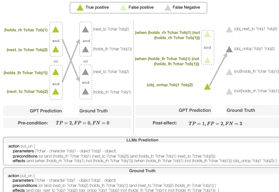
Figure 22: Transition Model evaluation metrics based on Bipartite Graph Matching for pre-conditions and post-effects.
