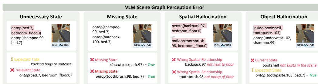
Figure 54: Possible VLM scene graph perception error types.
