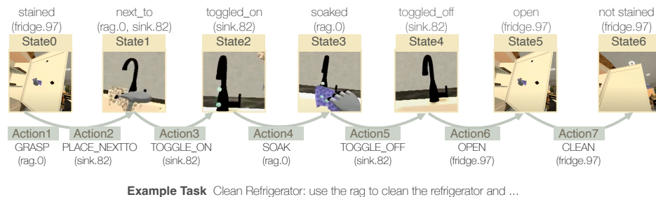
Figure 12: An example of successful execution in BEHAVIOR .
