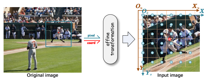
Figure A1: Pre-processing of NerPE. Due to differences in the affine transformations performed on pixels and coordinates, they are misaligned in the input image after standard data transformation. Therefore, we need to map the coordinates into O_u-X_u-Y_u to achieve alignment.
