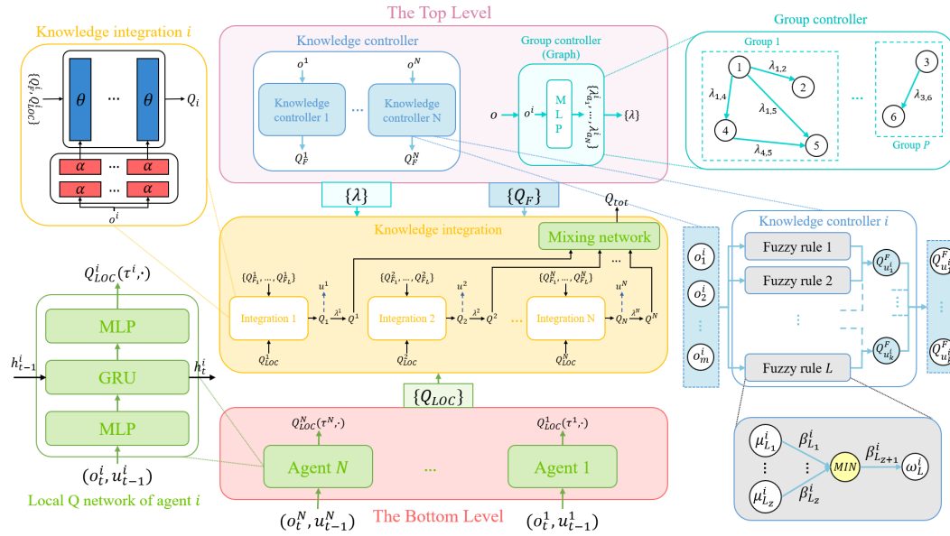
Figure 2: The overall framework of the human knowledge guided hierarchical MARL. The general architecture is proposed in the middle which is separated into three levels. Agents can develop their own policies with traditional MARL algorithm shown at bottom left. The graph-based group controller is depicted at top right to enhance agents' coordination. The knowledge controller is comprised with fuzzy logic rules to represent human knowledge which is demonstrated at bottom right. The hyper-networks of knowledge integration is illustrated at top left to allow agents freely decide the use of proposed human knowledge.
