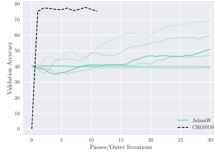
(b) CRONOS vs. AdamW trajectories on GPT2-NFT.
