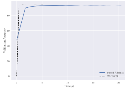
(c) CRONOS vs. tuned AdamW on GPT2-FT.
