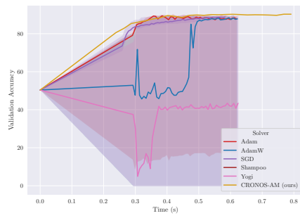
(a) CIFAR-10
