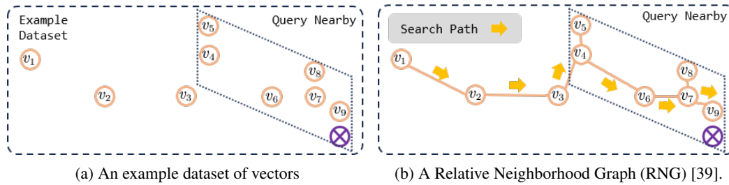
Figure 1: An example dataset of vectors and its proximity graph.
