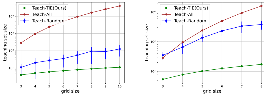
Figure 9: Performance of TIE compared to other baselines on visual programming task with local (on the left) and global features (on the right).
