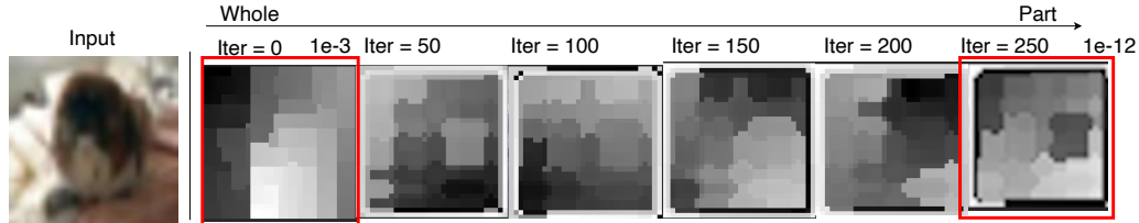
Figure 3: Overfitting on a single distilled token representation leads to islands of agreement[29] : APM is overfit on a test-sample’s representation distilled from a teacher. We plot t-sne clustering of output features over 250ttt iterations. L_2 loss between predicted features and distilled sample falls from 1e-3 to 1e-12 . Moving left to right shows that wholes break into smaller parts.
