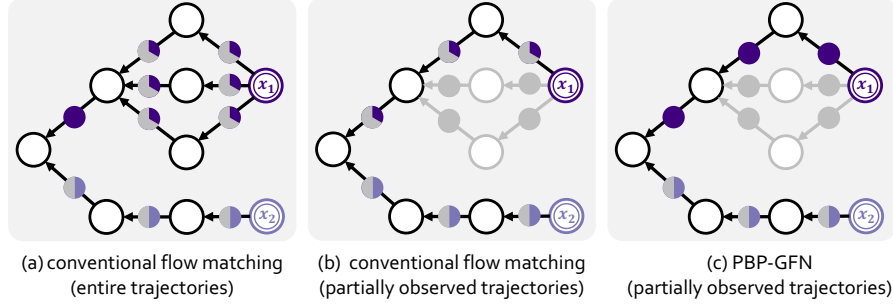
Figure 3: Pessimistic backward policy for GFlowNets (PBP-GFN). The portion of the circle indicates the amount of flow, e.g., \bullet indicates the flow of 1, and \circ indicates the half flow of \bullet , i.e., the flow of 0.5. Additionally, the color of the flow indicates the flow inducing the same-colored reward, and the black and gray lines indicate the observed and unobserved trajectories, respectively. (a) Flow matching succeeds with the entire trajectories. One can observe that the true reward of x_1 is 1 and the reward of x_2 is 0.5 by the amount of flow. (b) Flow matching fails with partially observed trajectories. (c) PBP-GFN assigns high probabilities to the backward transitions of observed trajectories to keep a high probability to high-reward objects.
