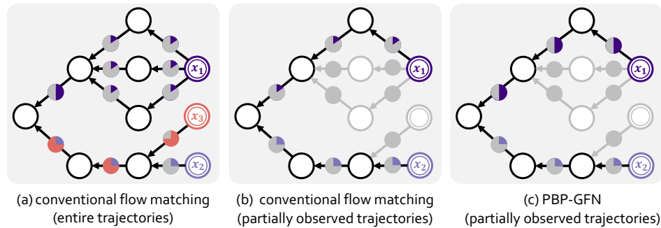
Figure 12: A synthetic example for the case where PBP-GFN may reduce exploration. The portion of the circle indicates the flow amount, and the color indicates the flow inducing the same-colored reward. The black and gray indicate the observed and unobserved trajectories, respectively. (a) The true reward of x_1 , x_2 , and x_3 are 0.5, 0.25, and 0.75, respectively. (b-c) Compared to the conventional GFN, PBP-GFN may yield a relatively low probability to the unobserved high-reward trajectory, by assigning a relatively high flow to the observed high-reward trajectory.
