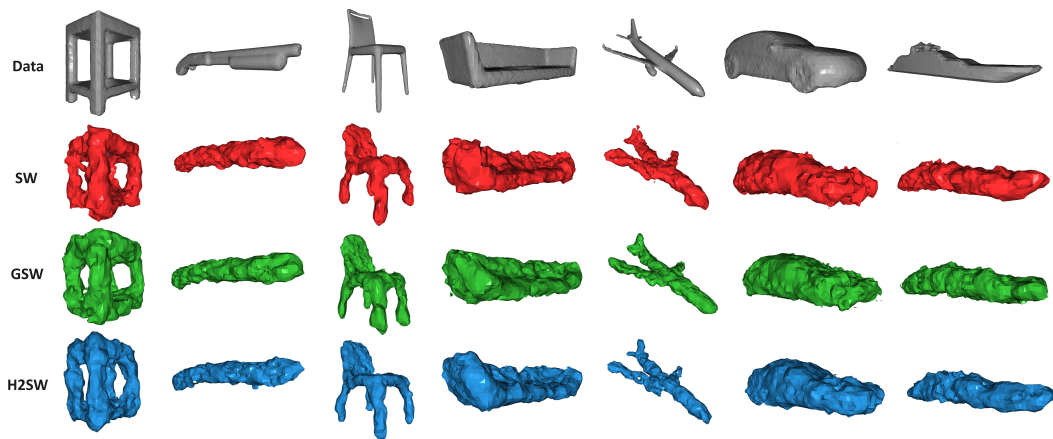
Figure 8: Visualization of some randomly selected reconstruction meshes from autoencoders trained by SW, GSW, and H2SW in turn with the number of projections L = 100 at epoch 500.
