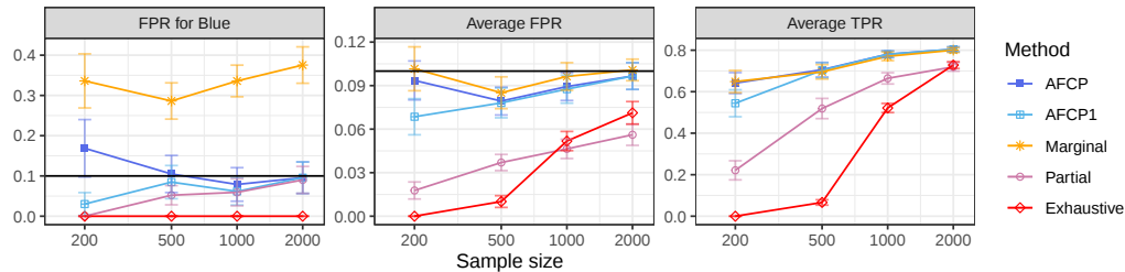
Figure A22: Performance on conformal p-values constructed by different methods on the synthetic data as a function of the total number of training and calibration points. Our method (AFCP) leads to higher TPR and lower FPR on the Blue group. The error bars indicate 2 standard errors.
