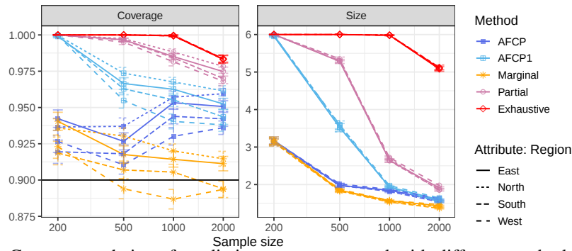
Figure A7: Coverage and size of prediction sets constructed with different methods for groups formed by Region. By design, all groups have similar performance, and none of them are subject to unfairness/undercoverage. See Table A8 for numerical details and standard errors.
