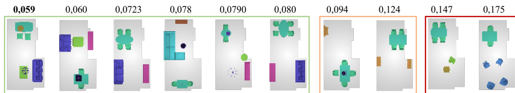
Figure 5: Top-down views of scenes generated by DeBaRA from several conditioning candidates provided by a LLM and their associated SSE values. We qualitatively observe that lower scores ( green ) corresponds to more natural layouts while higher scores ( red ) can be filtered out.
