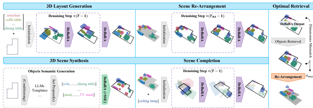
Figure 1: Application scenarios overview. Besides generating diverse and realistic 3D indoor layouts, a single trained DeBaRA model can be employed to execute several related tasks by tweaking the initial sampling noise level \sigma_{\max} and/or performing object or attribute-level layout inpainting. Our novel SSE procedure enables 3D Scene Synthesis capabilities by efficiently selecting conditioning semantics from external sources using density estimates provided by the pretrained model.
