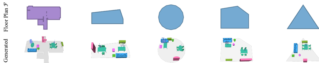
Figure 8: Generated layouts from a given set of objects and complex floor plans , selected from the 3D-FRONT test set or handcrafted to irregular, out-of-distribution shapes. While challenging, DeBaRA is able to output plausible layouts in which objects are scattered across the input floor plans.
