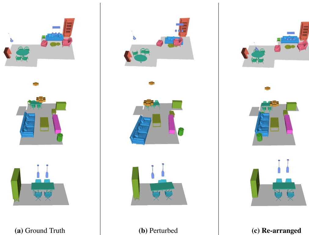
Figure 14: Additional re-arrangement results. Our method can recover a plausible arrangement from a noisy one using iterative sampling with fixed dimension attributes and low initial noise level.
