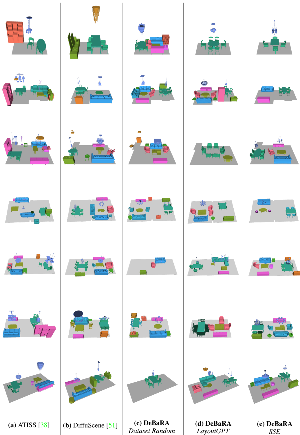
Figure 13: Additional scene synthesis results. We compare DeBaRA with state-of-the-art approaches in various settings. Since object semantics are not part of our output space, they are randomly drawn from the training dataset ( Dataset Random ), generated by an external LLM ( LayoutGPT ) or selected from LLM-generated sets by our density estimate procedure ( SSE ), which helps to get more natural layouts for the considered floor configuration.
