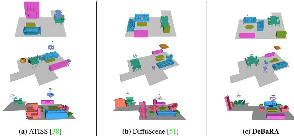
Figure 3: We compare our method with established baselines for generating a 3D layout from a floor plan and set of object categories. DeBaRA produces less failure cases while consistently generating regular arrangements within the room’s bounds.
