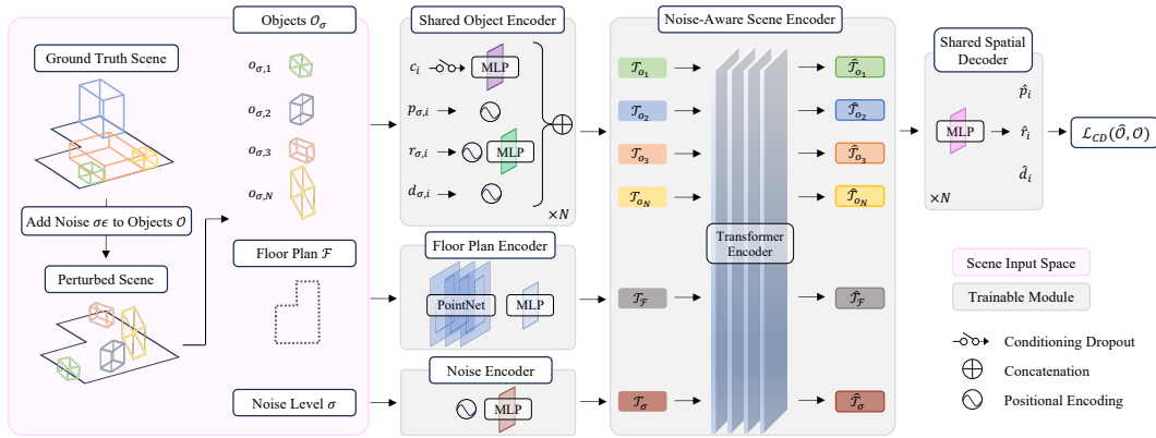
Figure 2: DeBaRA architecture and training overview. At each iteration, 3D bounding boxes parameters (p, r, d) of indoor scene’s objects \mathcal{O} are perturbed with Gaussian noise \sigma\epsilon . The floor plan \mathcal{F} , noise level \sigma and resulting objects \mathcal{O}_\sigma are processed by respective encoders to form an unordered set of representations \mathcal{T} fed as input to a transformer encoder. Novel object embeddings \hat{\mathcal{T}}_o are finally decoded back to their predicted clean spatial configuration (\hat{p}, \hat{r}, \hat{d}) . Trainable modules are optimized by minimizing a semantic-aware Chamfer loss. Input object categories c are randomly dropped to model both the class-conditional and unconditional 3D layout distributions.
