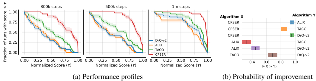
Figure 15: Performance profiles and probabilities of improvement of different methods.
