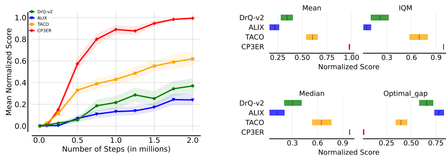
Figure 6: Results on Meta-world tasks with 5 random seeds.
