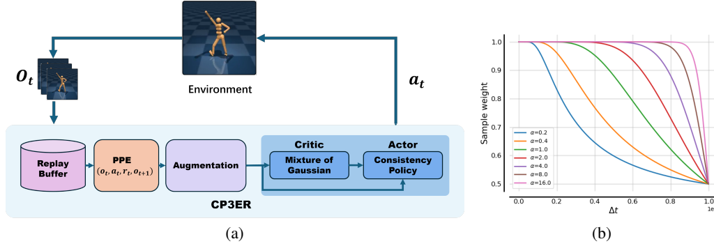
Figure 3: (a) The framework of CP3ER, where PPE is the abbreviation of prioritized proximal experience. (b) The sampling weights \beta with different \alpha .
