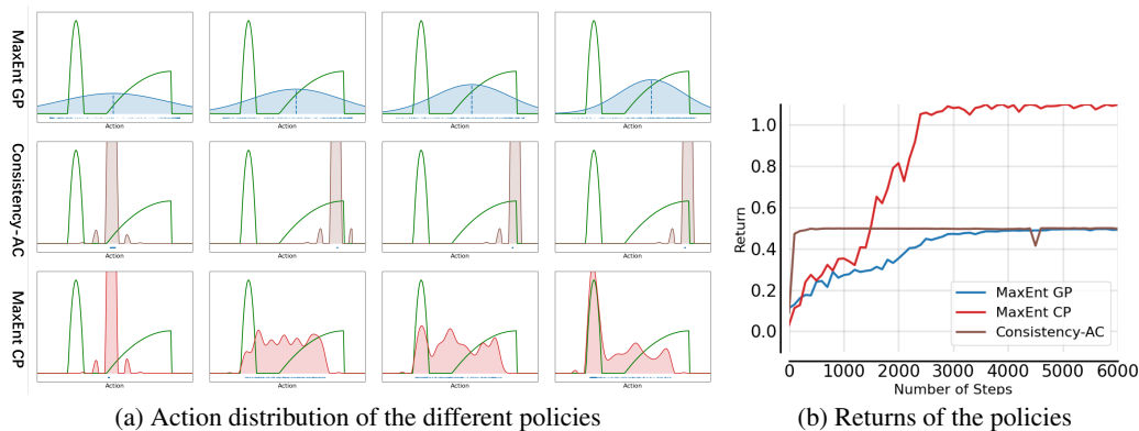
Figure 7: Results on the toy example. Left part is action distributions during training, while right is returns of different policies.
