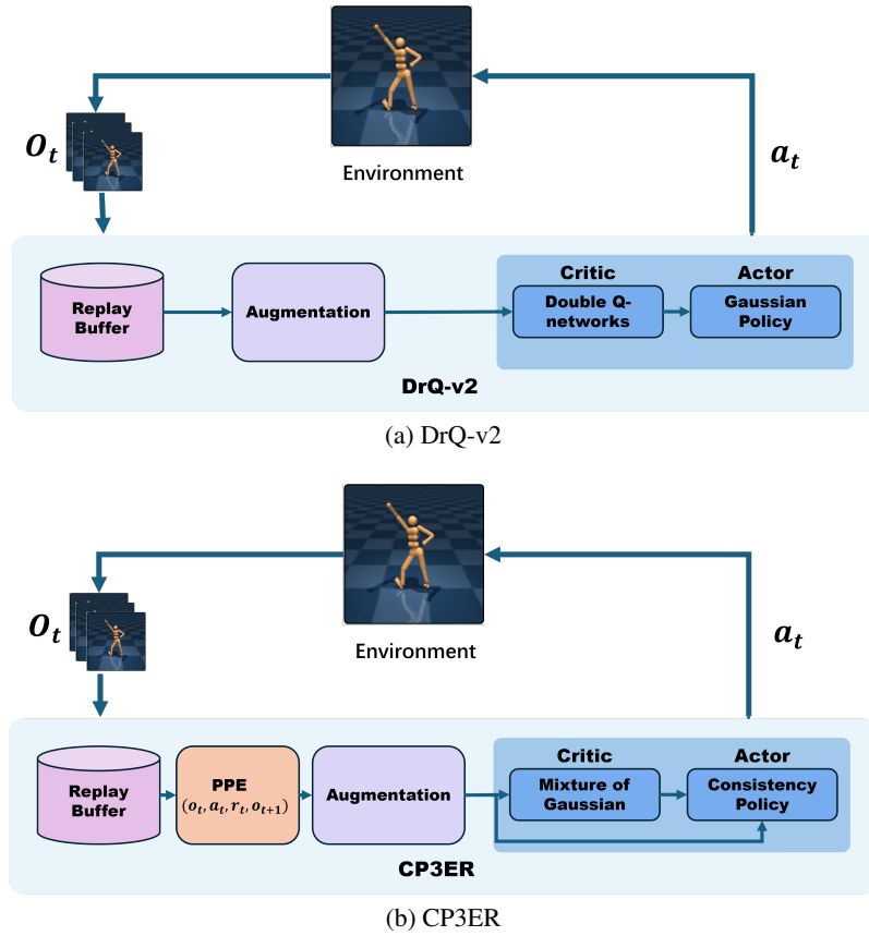
Figure 13: Comparison between DrQ-v2 and CP3ER.
