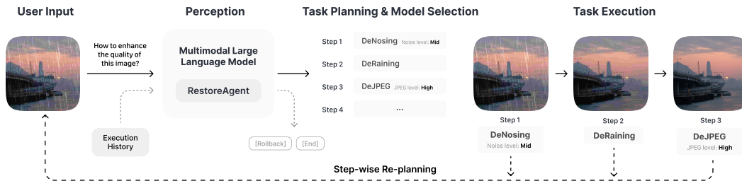
Figure 3: Illustration of the data construction workflow and RestoreAgent pipeline.
