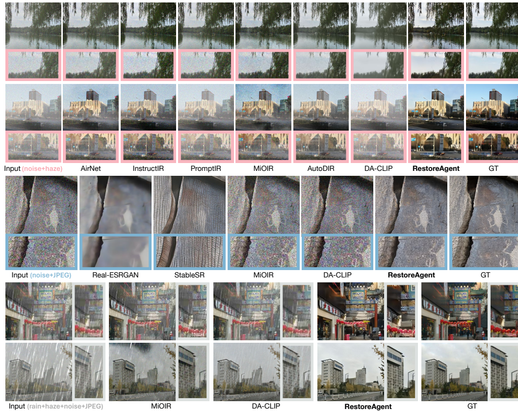
Figure 5: Visual comparisons with All-in-One Methods. To ensure a fair comparison, All-in-One methods are tested only on the degradation types and datasets they support. The all-in-one approach still lacks the ability to effectively handle images containing multiple types of degradation.
