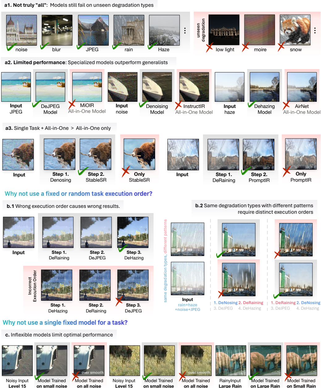
Figure 2: Limitation illustration of all-in-one models, fixed task execution order, and fixed model. Images with a pink background indicate negative examples
