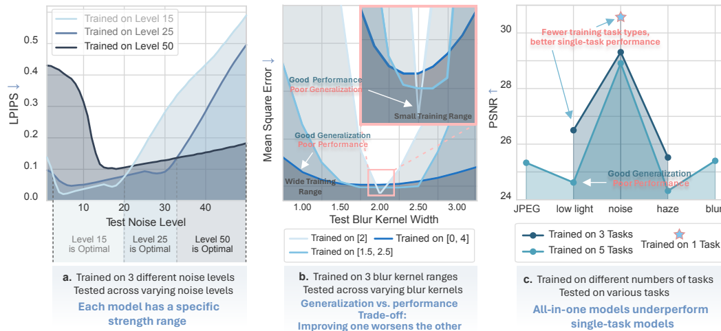
Figure 1: Limitations of all-in-one models. (a) Models trained on different noise levels excel in specific areas, so choosing models on demand leads to better results. (b) Models trained on a wider range of blur degradations offer improved generalization but compromised performance, showing a trade-off. (c) Multi-task models underperform on individual tasks compared to single-task models, illustrating that all-in-one models trade performance for generalization.
