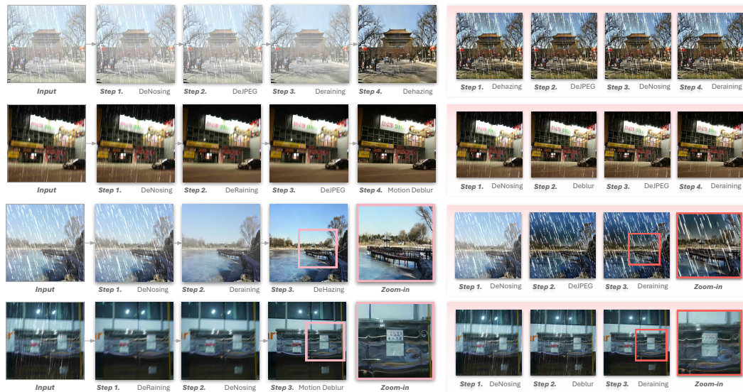
Figure 4: Illustrations of RestoreAgent's choices demonstrate that our approach predicts the correct task sequence. Images with a pink background show inappropriate decisions.
