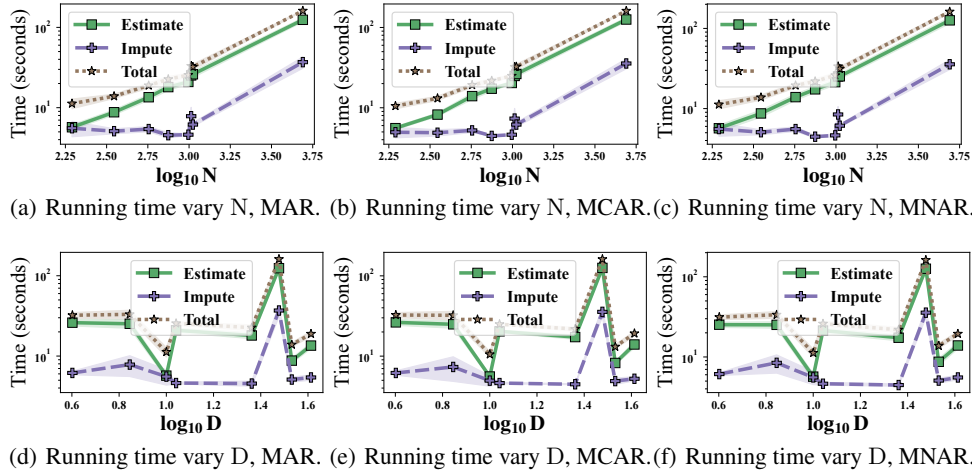
Figure F.3: Average computation time, where ‘Estimate’ indicates the ‘DSM Training Algorithm’ (step 5 of Algorithm 1), and ‘Impute’ indicates the imputation algorithm (step 7 of Algorithm 1). The scatters and shaded areas indicate the mean and one standard deviation from the mean, respectively.
