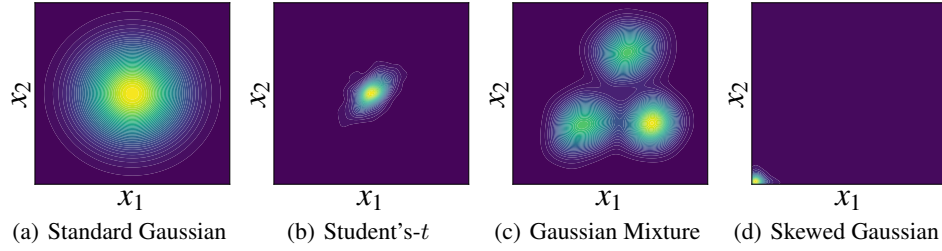
Figure F.1: Contours of Various Distributions' Density Value.
