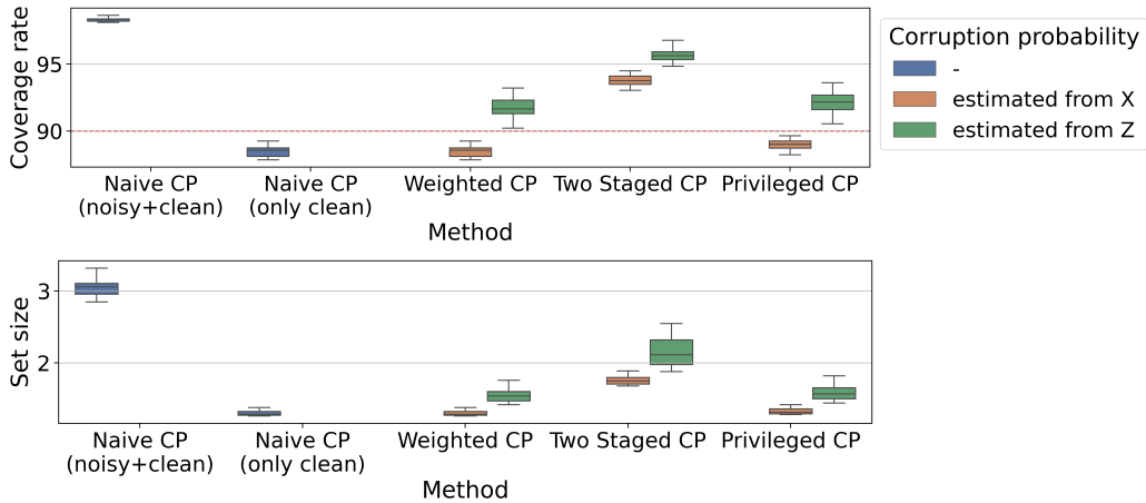
Figure 7: Noisy response experiment: CIFAR-10N dataset. The coverage rate and average set size length achieved by, naive conformal prediction (Naive CP), using either all calibration samples (noisy + clean) or only the uncorrupted ones (only clean), Weighted CP which estimates the corruption probability from either X (orange), Z (green), the baseline Two Staged CP and the proposed method (Privileged CP) with the two options for the corruption probabilities. All methods are applied to attain a coverage rate at level 1 - \alpha = 90\% . The metrics are evaluated over 20 random data splits.
