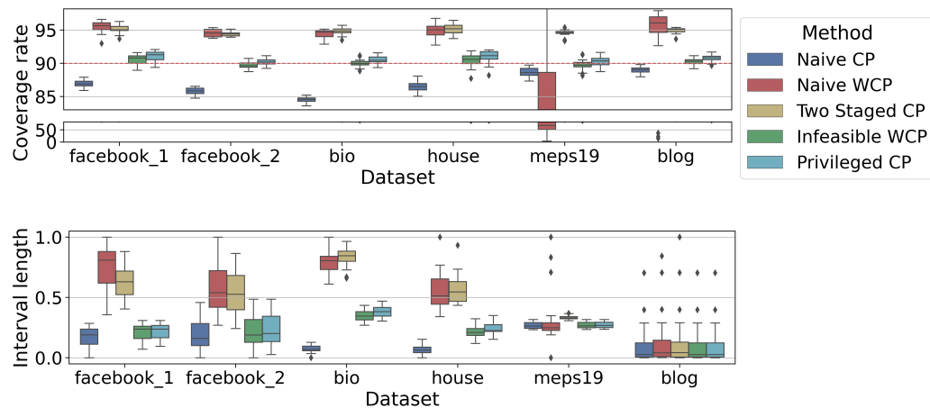
Figure 2: Missing response experiment. The coverage rate and average interval length obtained by various methods; see text for details. Performance metrics are evaluated over 20 random data splits.
