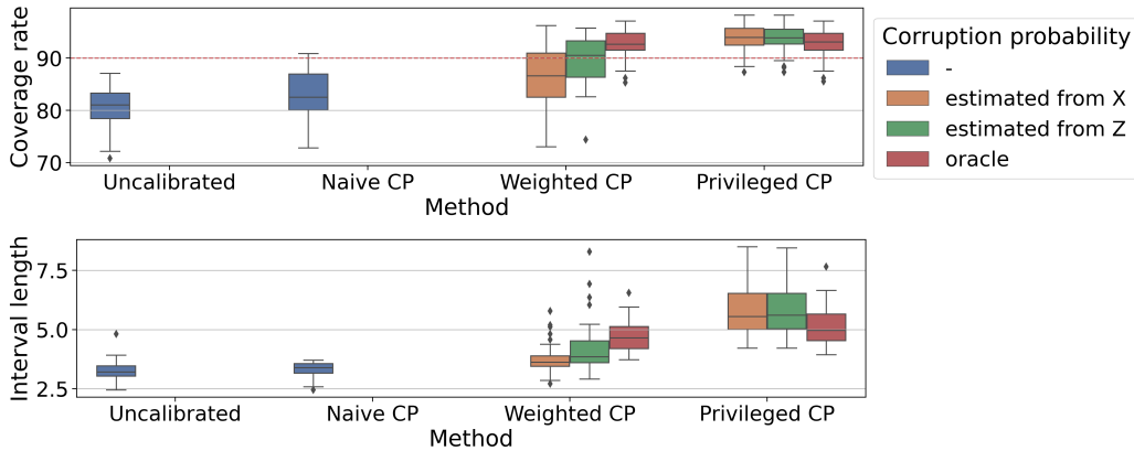
Figure 4: IHDP dataset experiment. The coverage rate and average interval length achieved by an uncalibrated quantile regression (Uncalibrated), a naive jackknife+ (Naive CP), JAW (Weighted CP) which estimates the corruption probability from either X (orange), Z (green), or uses the oracle probabilities (red), and the proposed method (Privileged CP) with the three options for the corruption probabilities. All methods are applied to attain a coverage rate at level 1 - 2\alpha = 90\% . The metrics are evaluated over 50 random data splits.
