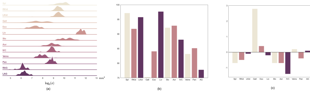
Figure 14: (a) The organ volume statistics of BTCV training dataset. (b) Class-wise Dice of nnUNet (visualization of Table 11). Note that AG denotes the average of the right and left adrenal glands (RAG and LAG). (c) Class-wise Dice differences between E2ENet with feature sparsity 0.7 and nnUNet on BTCV test dataset. The positive value means that E2ENet outperforms nnUNet, and vice versa.
