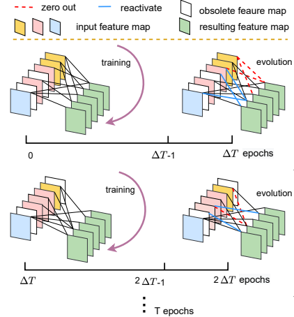
Figure 3: Illustration of our Dynamic Sparse Feature Fusion (DSFF) mechanism. The fusion operation starts from sparse feature connections and allows the connectivity to be evolved after training for \Delta T epochs. During each evolution stage, a fraction of kernels with smaller L_1 norms will be zeroed out (red dotted line), while the same fraction of other inactivated connections will be reactivated randomly, keeping the feature sparsity S constant during training (blue solid line).
