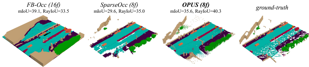
Figure 3: Visualizations of occupancy predictions. Best viewed in color.
