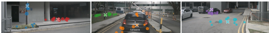
Figure 7: the self-attention in decoders. for each pivot (marked as \times ), query points with top 10 attention weights are shown by circles, with sizes proportional to weights. best viewed in color.
