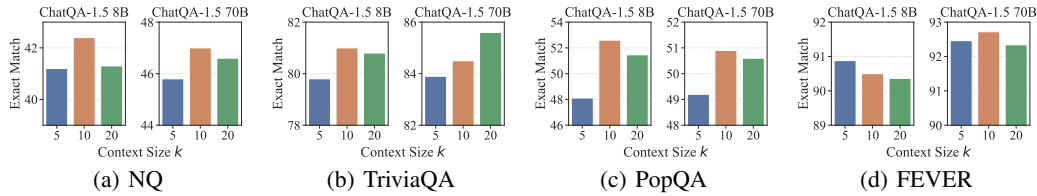
Figure 1: Performance of ChatQA-1.5, one of the strongest RAG models, on different context size k . We observe a trade-off of selecting top- k contexts: a smaller k compromises the recall, while a larger k could introduce irrelevant or noisy context and mislead the LLM generation.
