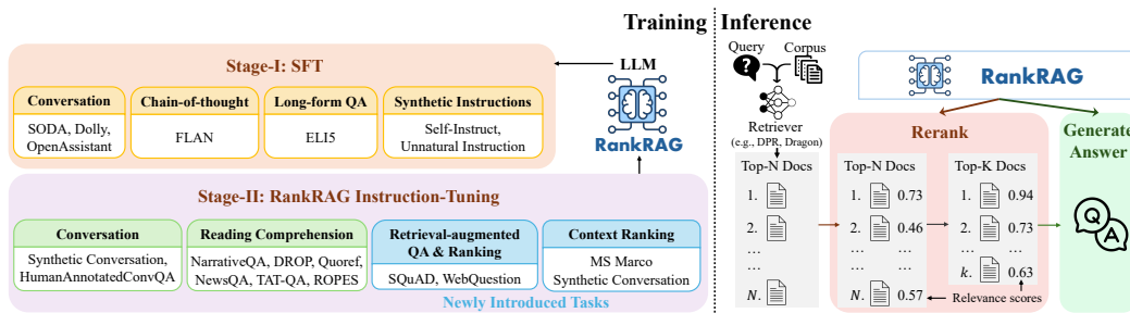
Figure 2: Two-stage instruction tuning framework for RankRAG.
