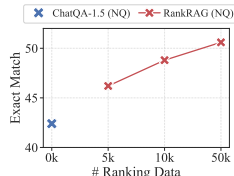
Figure 4: Performance w.r.t. # Ranking Data
