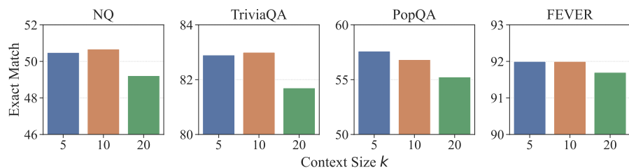
Figure 6: Performance of RankRAG on different context size k .
