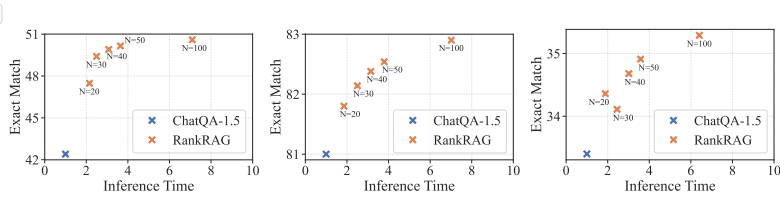
(a) NQ (b) TriviaQA (c) HotpotQA Figure 5: Performance v.s. Efficiency analysis for RankRAG.
