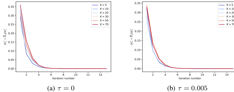
Figure 2: Changing map size K . we let \tau = 0, 0.005 and change K for each \tau . We plot the curves of (V_t^* - \bar{V}_t^{(t)})/V_t^* changing with the iteration number. We can see that both vanilla and entropy-regularized NPG converges to the optimal value function in a few iterations, and the convergence speed is almost the same across different K .
