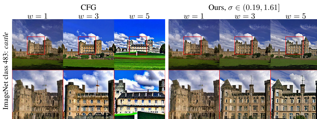
Figure 9: Effect of increasing guidance weight w with CFG vs. our method. Left: Increasing the guidance weight with CFG leads to changes in image composition and contrast. Right: With our method, increasing w improves image details but retains the overall composition and realistic colors.
