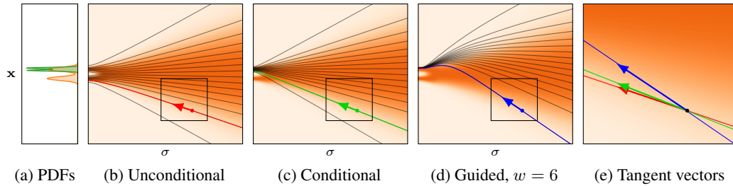
Figure 1: Visualizing the effect of guidance. (a) The unconditional (orange) and conditional (green) PDFs. In (b) through (e) , the orange unconditional density is visualized in the background. (b) Sample trajectories for the unconditional distribution. (c) Trajectories for the conditional distribution. (d) Trajectories for the guided distribution with w = 6 . (e) The tangent vectors dx/d\sigma at the intersection point of the three marked trajectories. The difference of the unconditional (red) and conditional (green) vectors is magnified as per Equation 4, causing the unexpected detour in low-probability areas and a mode drop. See Figure 2 for details and comparison to our approach.
