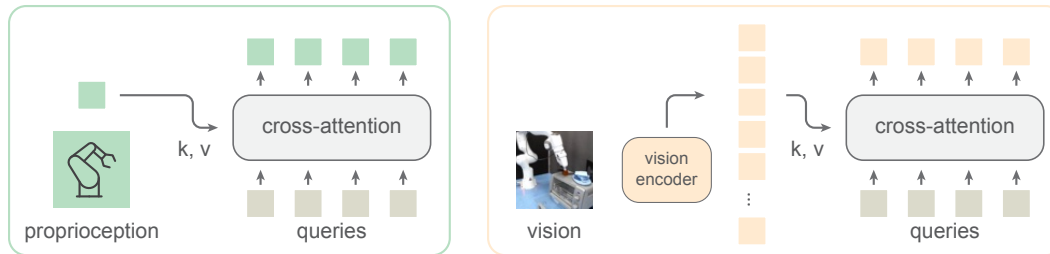
Figure 3: Stem Architecture in HPT. In the HPT stem, the proprioceptive tokenizer uses an MLP to map proprioceptive information to a feature which is then attended by 16 learnable tokens. The vision tokenizer uses pre-trained encoders and similarly uses an attention mechanism to map vision features into 16 fixed tokens. The architecture flexibly handles sequences of inputs without increasing the size of tokens.
