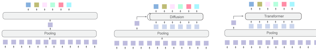
Figure 14: Flexible Head Architectures in HPT. We highlight that our HPT architecture is a meta-level architecture for policy learning, and it can work with various head architectures. The important takeaway is the scalable transformer architecture in the middle of the policy to absorb the diverse data and provide tokens for these policy heads to regress on the action outputs.
