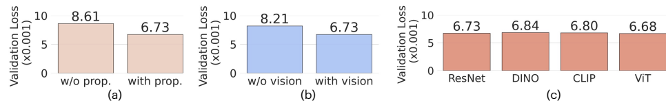
Figure 18: Ablation Study on HPT Stem. We ablate the pre-training performance for (a) proprioception, (b) vision stems, and (c) vision encoders. Setting: HPT-S, batch 256, iterations 80000, 27 datasets with a maximum of 1000 trajectories for each dataset.
