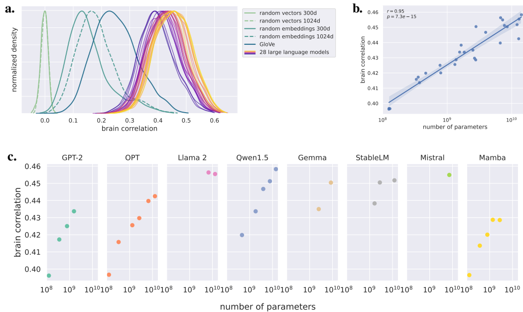
Figure 2: Performance of various models in predicting fMRI brain time-courses. (a) Density estimates of the distributions of r -scores obtained for all 28 large language models, the random baselines and GloVe. The densities are scaled to have the same maximum (b) Average r -score as a function of the number of parameters of the model, in log scale. Here and in the next figures, the shaded area indicates the 95% confidence interval of the slope, computed with bootstrap. (c) Same, split by models' family.
