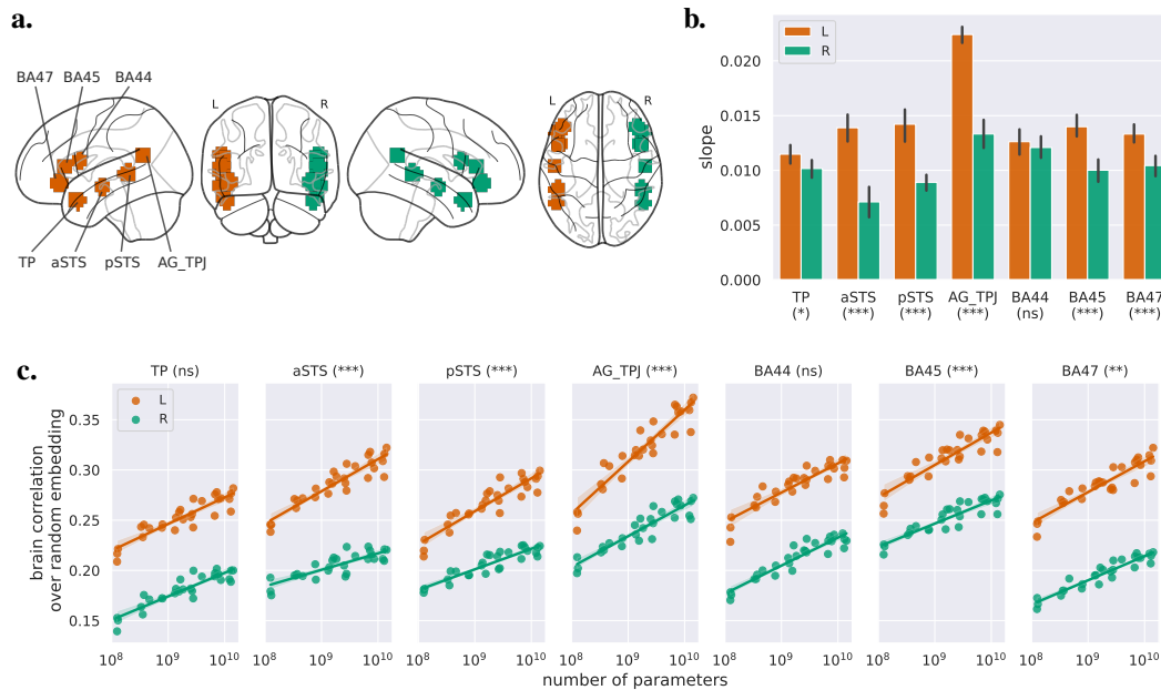
Figure 7: Model size impact in various Regions of Interest. (a) Locations of ROIs. (b) Slope in r -score as a function of the logarithm of the number of parameters, averaged over all voxels of a given ROI. Error bars indicate 95% confidence interval, estimated by bootstrap. The annotation below each ROI label indicates an estimate of the level of statistical significance of the difference between the slopes of the voxels of a left ROI compared to its respective right ROI (ns: non significant, *: p < 0.05 , **: p < 0.01 , ***: p < 0.001 ). (c) Brain correlations over the random embedding baseline (see Fig. B.9 on page 22 for similar plots with raw brain correlations), as a function of the logarithm of the number of parameters. The annotation next to each ROI label indicates the level of statistical significance of the correlation between the models on the left hemisphere minus the right hemisphere, as a function of the logarithm of the number of parameters, testing the interaction between hemisphere and model size. See Table A.2 for full statistics.
