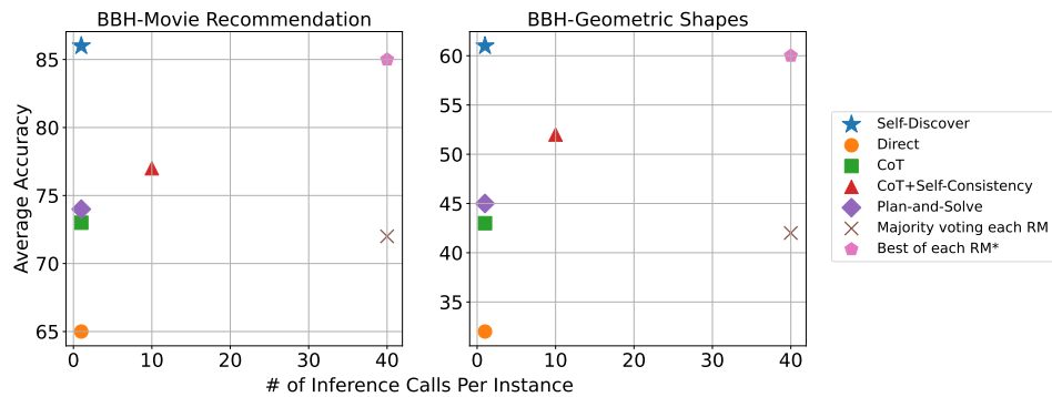
Figure 5: Comparison of accuracy with number of inference calls required per instance. For CoT-Self-Consistency, we sample 10 times. Best of each RM method requires gold labels (*). SELF-DISCOVER requires only 1 inference call per instance, same as Direct and CoT while reaching better performance compared with 40x more call required methods on GPT-4. We acknowledge that SELF-DISCOVER input and output are longer than CoT and Direct prompting, increasing cost. However, as the number of instances increases, the efficiency of SELF-DISCOVER in terms of inference per instance is highly desirable.
