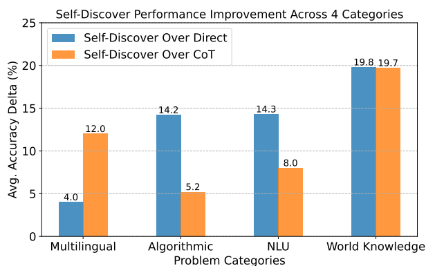
Figure 4: Breakdown of SELF-DISCOVER performance improvement on 4 categories on PaLM 2-L. SELF-DISCOVER performs the best on tasks requiring world knowledge.
