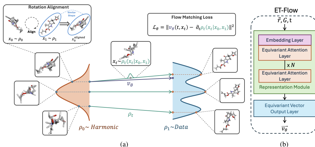
Figure 1: (a) Overview of ET-Flow. The model predicts a conditional vector field \vec{v}_\theta using interpolated positions ( x_t ), molecular structure ( G ), and time-step ( t ). Samples are drawn from the harmonic prior ( x_0 \sim p_0 ) and then rotationally aligned with the samples from data ( x_1 \sim p_1 ). A conditional probability path is constructed between pairs of x_0 and x_1 , and x_t is then sampled from this path at a random time t . (b) The ET-Flow architecture consists of a representation module based on the TorchMD-NET architecture (Thölke and De Fabritiis, 2022) and an equivariant vector output module. For detailed architecture and input preprocessing information, see Section A.1.
