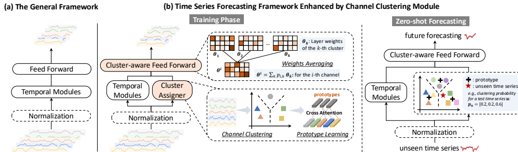
Figure 1: The pipeline of applying Channel Clustering Module (CCM) to general time series models. (a) is the general framework of most time series models. (b) illustrates two modified modules when applying CCM: Cluster Assigner and Cluster-aware Feed Forward. Cluster Assigner learns channel clustering based on intrinsic similarities and creates prototype embeddings for each cluster via a cross-attention mechanism. The clustering probabilities \{p_{i,k}\} are subsequently used in Cluster-aware Feed Forward to average \{\theta_k\}_{k=1}^K , which are layer weights assigned to K clusters, obtaining weights \theta^i for the i -th channel. The learned prototypes retain pre-trained knowledge, enabling zero-shot forecasting on unseen samples in both univariate and multivariate scenarios.
