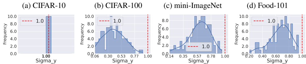
Figure 3: Verification of condition numbers \{\sigma_y\}_{y=1}^K in Equation 6 with imbalance type EXP, \rho = 0.1 when \alpha = 0.1 and models are trained with 200 epochs. Vertical dashed lines represent the value 1, and we observe that all the condition numbers are smaller than 1. This verifies the validity of the condition for Lemma 4.2, and thus confirms that RC3P produces smaller prediction sets than CCP using calibration on both non-conformity scores and label ranks.
