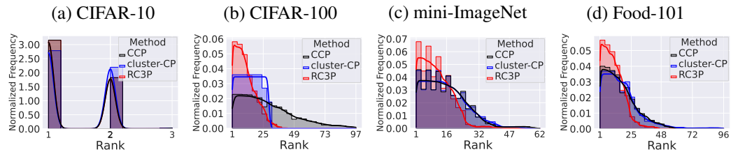
Figure 10: Visualization for the normalized frequency distribution of label ranks included in the prediction set of CCP, Cluster-CP, and RC3P with \rho = 0.5 EXP when \alpha = 0.1 . It is clear that the distribution of normalized frequency generated by RC3P tends to be lower compared to those produced by CCP and Cluster-CP. Furthermore, the probability density function tail for label ranks in the RC3P prediction set is notably shorter than that of other methods.
