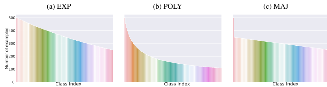
Figure 4: Illustrative examples of the different imbalanced distributions of the number of training examples per class index c on CIFAR-100
