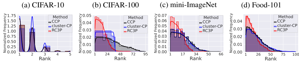
Figure 2: Visualization for the normalized frequency distribution of label ranks included in the prediction set of CCP, Cluster-CP, and RC3P with \rho = 0.1 for imbalance type EXP when \alpha = 0.1 and models are trained with 200 epochs. It is clear that the distribution of normalized frequency generated by RC3P tends to be lower compared to those produced by CCP and Cluster-CP. Furthermore, the probability density function tail for label ranks in the RC3P prediction set is notably shorter than that of other methods.
