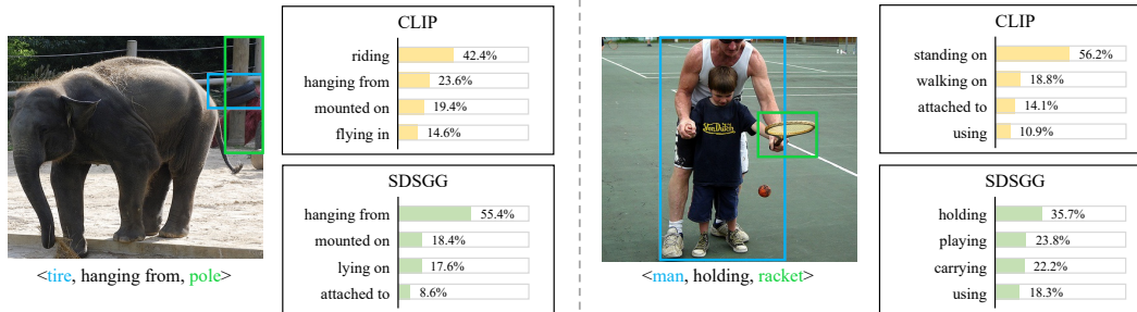
Figure 3: Visual results (§4.3) on VG [14].
