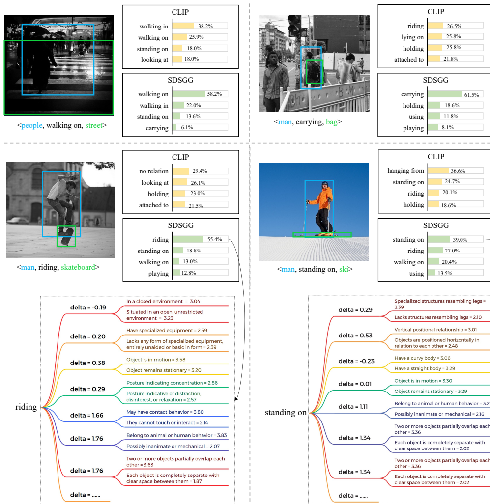
Figure S6: Visual results (§E) on VG [14] test. As seen, SDSGG makes the right predictions based upon the scene-specific descriptions and self-normalized similarities.
