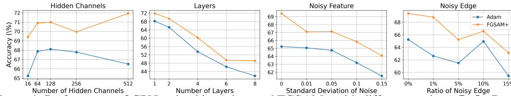
Figure 4: Performance of GPN trained by Adam and FGSAM+ with different settings. Left: Results with various hidden channels. Middle Left: Results with various model depths. Middle Right: Results with features perturbed by noise of varying standard deviations. Right: Results with edges subjected to various noise ratios.
