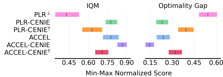
Figure 10: IQM and Optimality Gap ablations in Minigrid domain. Results are measured across 5 independent runs.
