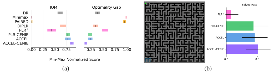
Figure 3: (a) Aggregate zero-shot transfer performance in Minigrid domain across 5 independent runs. (b) Zero-shot test performance of \text{PLR}^\perp , PLR-CENIE, ACCEL, and ACCEL-CENIE on PerfectMazeLarge across 5 independent runs.
