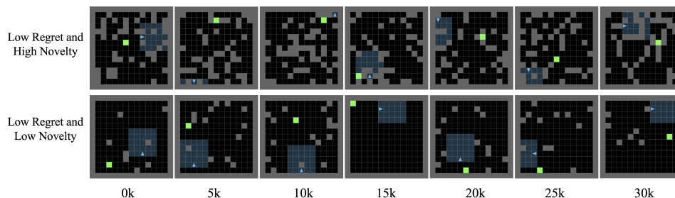
Figure 11: Levels in the level replay buffer of \text{PLR-CENIE} . X-axis: number of student PPO updates.
