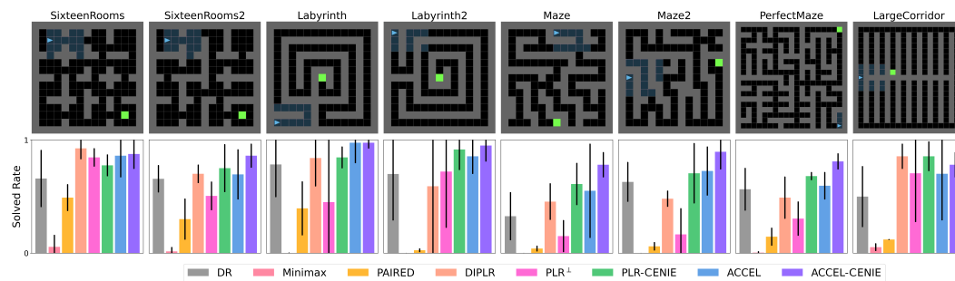
Figure 2: Zero-shot transfer performance in eight human-designed test environments. The plots are based on the median and interquartile range of solved rates across 5 independent runs.
