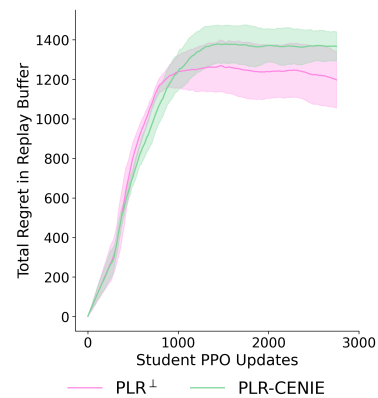
Figure 8: Total regret in level replay buffer for PLR ⊥ and PLR-CENIE over training in CarRacing.
