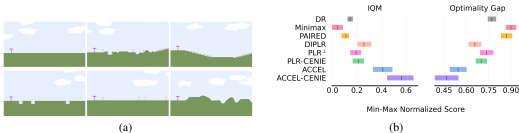
Figure 6: (a) BipedalWalker domain and (b) Aggregate zero-shot transfer performance in BipedalWalker.
